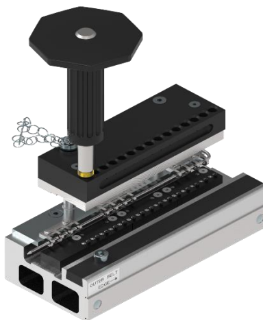
Installation Unit H24 Profi 15-180
